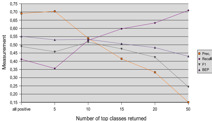
Fig. 1. Rank strategy results for PLAUM algorithm
