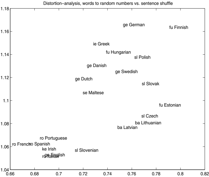
Fig. 4. Morphological and syntactic complexity of the languages in a two-dimensional graph
