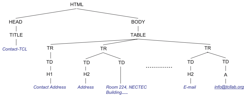
Fig. 2. An example of HTML tag tree
