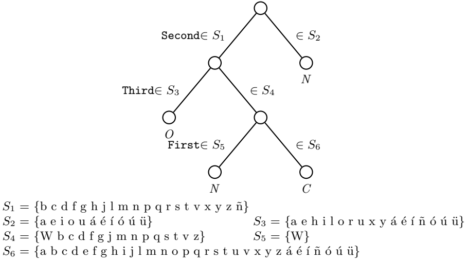
Fig. 1. Classification tree trained with 4000 words of Benedetti
