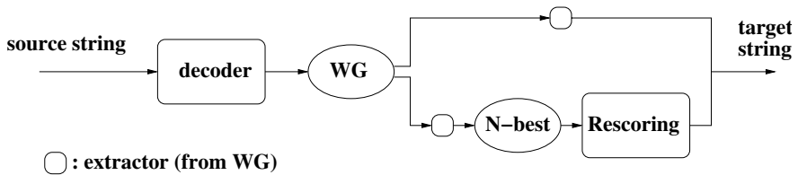
Fig. 1. Architecture of the ITC-first SMT system. The decoder produces a word-graph (WG) of translation hypotheses. In single-stage translation the most probable string is output. In two-stage decoding, N-best translations are extracted, re-scored, and re-ranked by applying additional feature functions.
