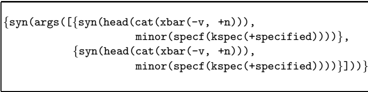
Fig. 4. Arguments of a transitive verb
