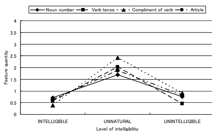
Fig. 4. Grammatical Errors
