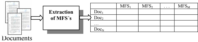
Fig. 1. Proposed representation
