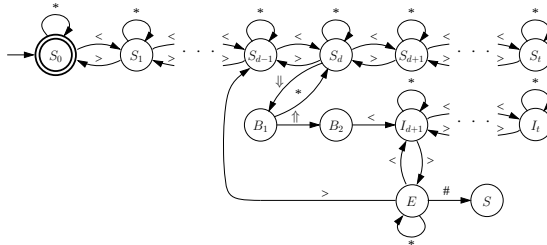
Fig. 6. Connectivity FSA C_{d,t} . The states S_0 – S_d maintain balanced bracketing up to the depth d . If the current word is a left-bare word at depth d , the FSA reaches state B_2 , otherwise it returns to state S_d . States I_{d+1} – I_t maintain a balanced bracketing from the left-bare word onward and the state E is reached upon closing the depth d . If, at this point, also the depth d - 1 is closed, it means that the left-bare word did not open an island since the current depth is smaller than d . The FSA then returns to state S_{d-1} . If, on the other hand, the FSA proceeds from the state E to S , it has reached a right-bare word and the depth within the island was never been smaller than d . Therefore, an island was found and since S is a sink state, the string is rejected.
