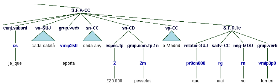
Fig. 2. Constituent discontinuity
