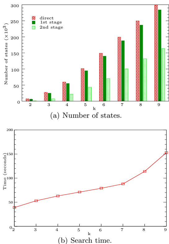
Fig. 2. Spatial and temporal costs. Figure 2(a) The size, in terms of number of states, of k-TSS models for several values of k; the first column refers to the direct model, and the second and third to the two-stage model. Figure 2(b) The translation time for 1,500 test sentences.
