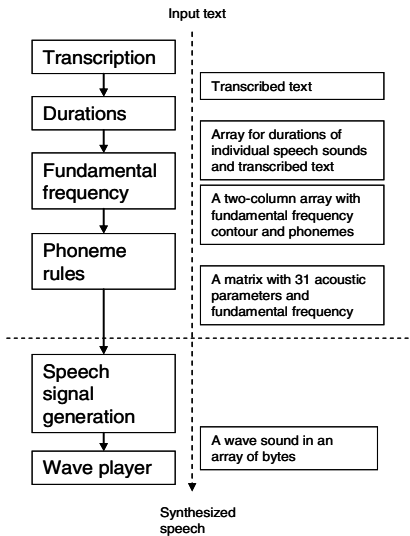
Fig. 1. The structure of the software is divided into two phases; the high-level synthesizer and the signal generation, which are separated by a horizontal dashed line. Each step in the synthesizing procedure is shown on the left and the changes in the information state is described on the right.
