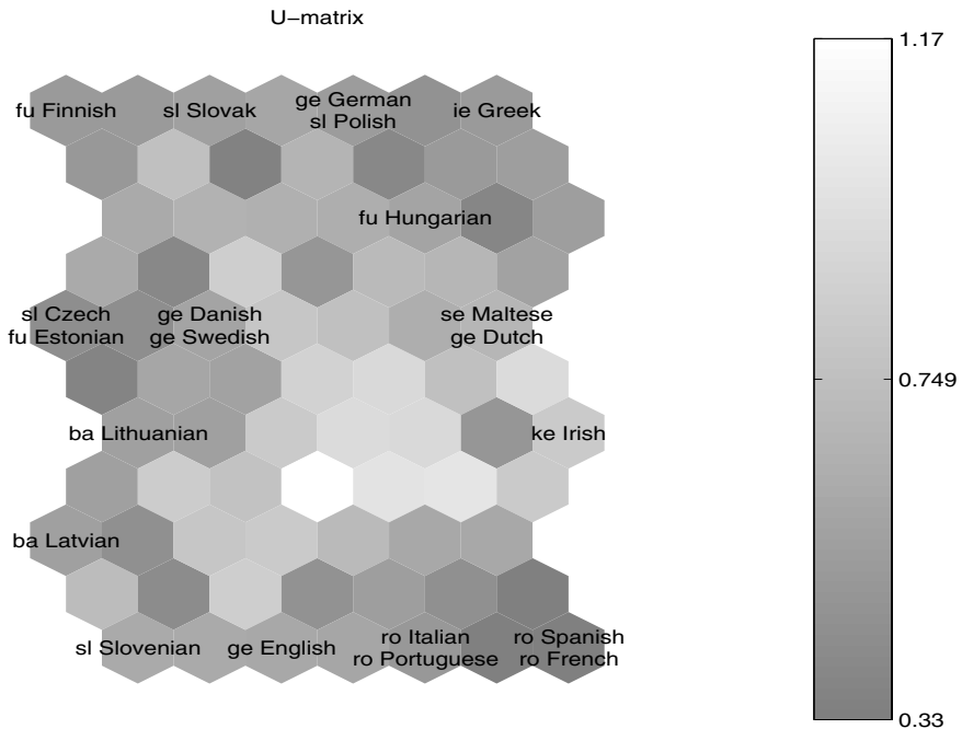
Fig. 5. Languages in a SOM-map: morphology vs. word order information
