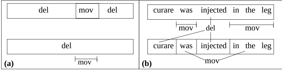
Fig. 3. (a): Decorator transformation, (b): Block split
